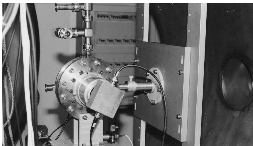
FIGURE 3. A picture of the apparatus.
